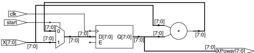
Figure 1.1 Iterative implementation.
