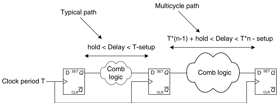
Figure 18.4 Multicycle path.
