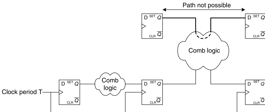
Figure 18.5 False path.
