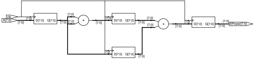
Figure 1.2 Pipelined implementation.
